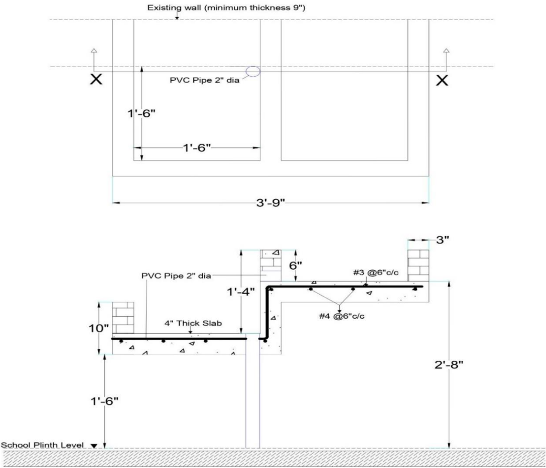
PLAN & X-SECTION of Hand Wash Facility
