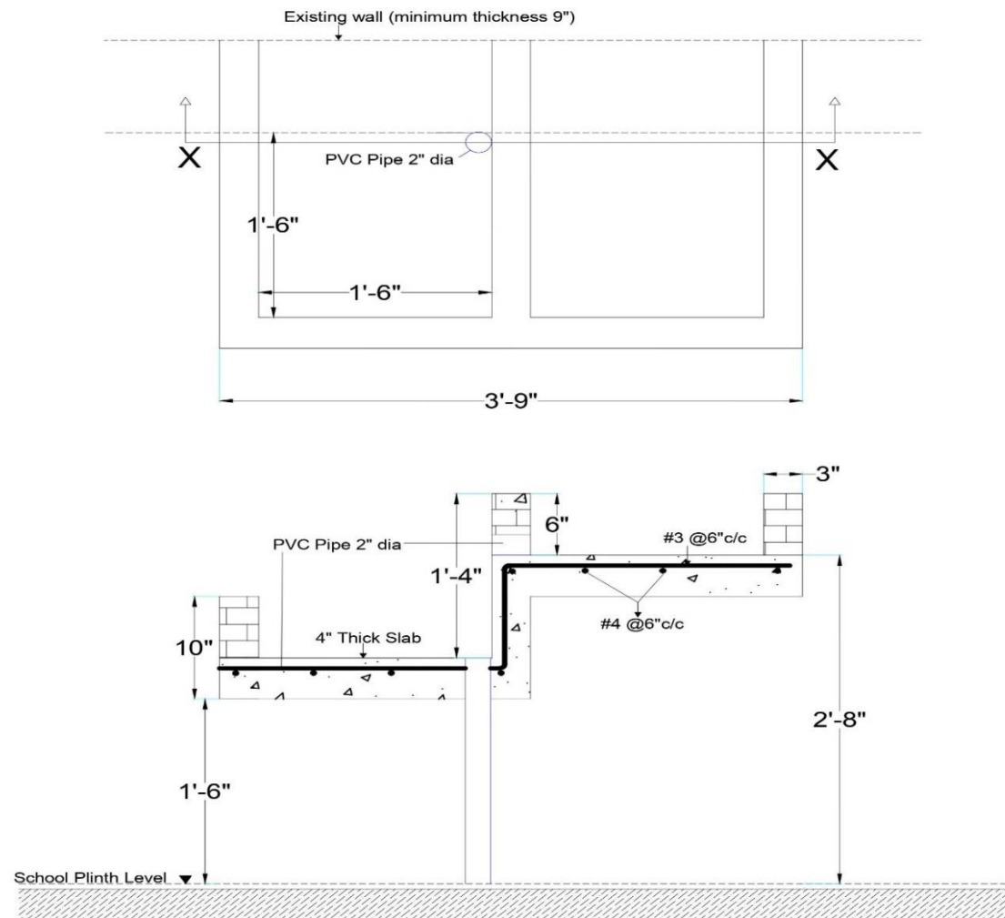
PLAN & X-SECTION of Hand Wash Facility
