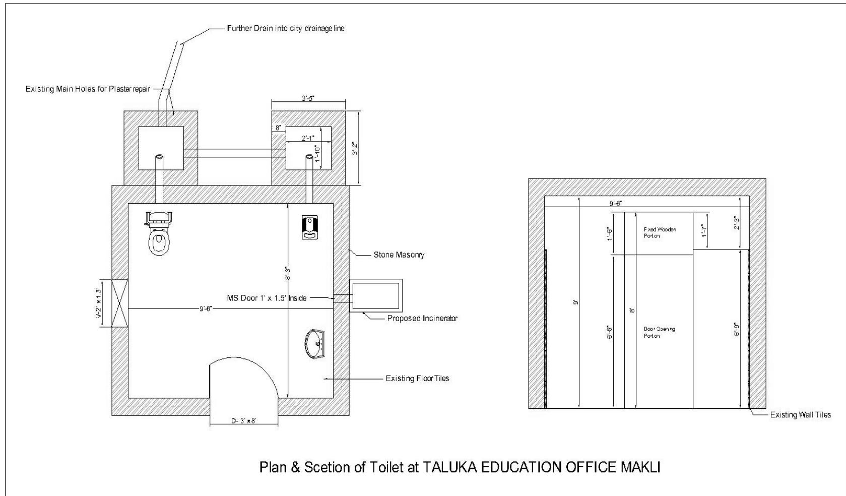
Rehabilitation Detailed Drawings Site 04: Rehabilitation Plan of Latrine
