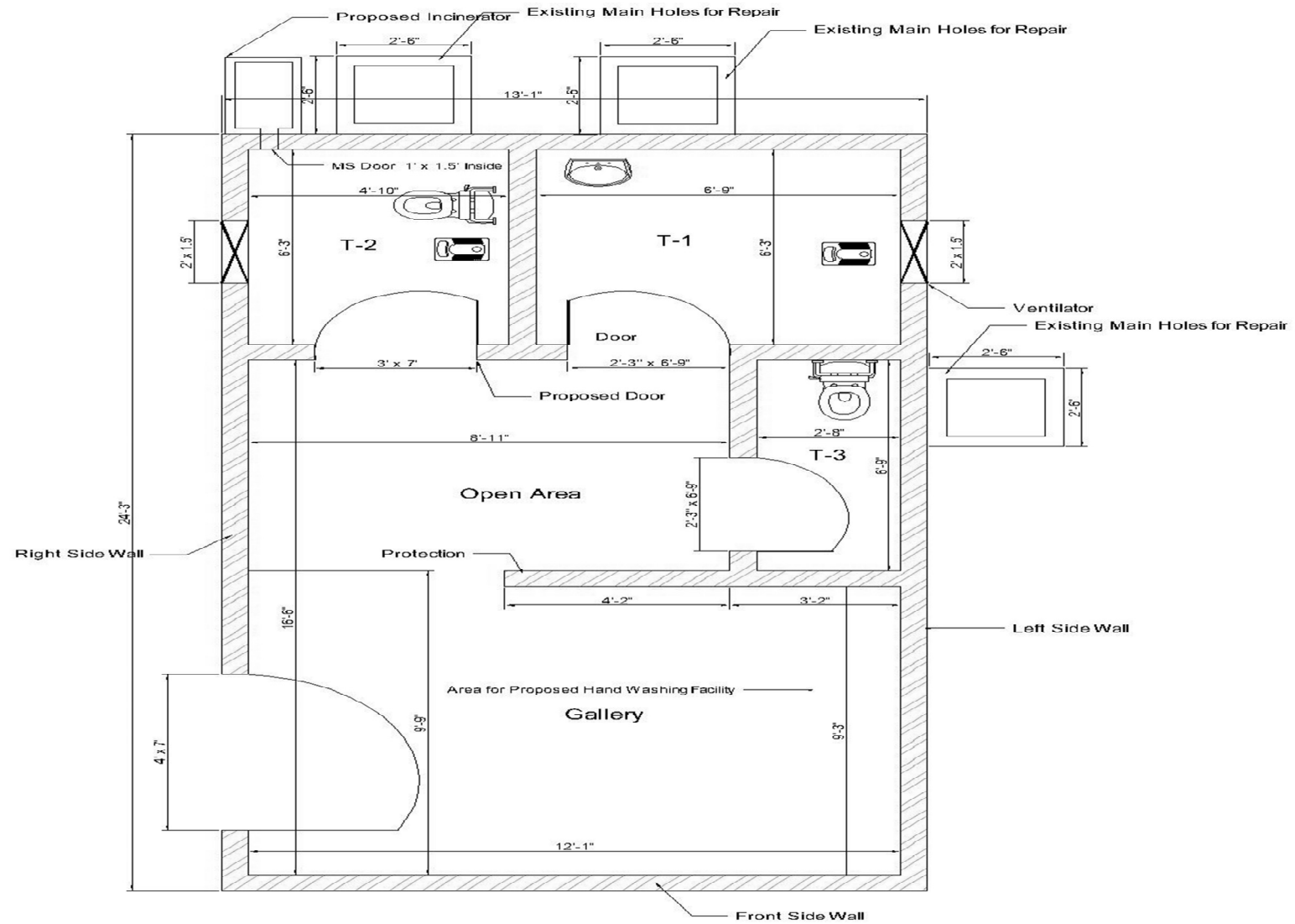
Plan of Toilet of Civil Hospital Makli (Portion-1)
